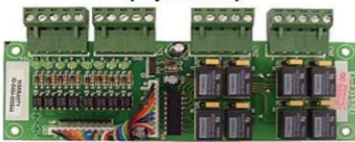
ECL-ACC1010 I/O Expansion 8 DI & 8 DO Board Ethernet Interface 10 Base-T (Optional)
